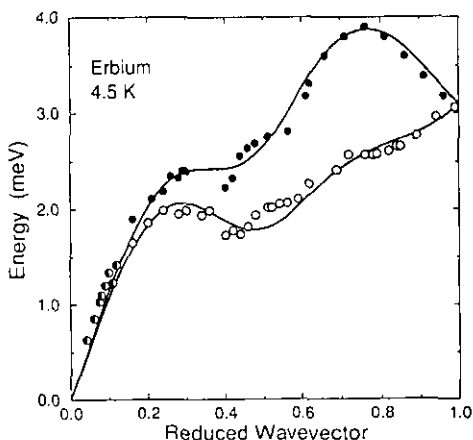
Figure 5. Spin-wave dispersion relations in the c -direction in the cone phase of erbium at 4.5 K. The closed and open circles represent the measured +q and -q branches, respectively (Nicklow et al 1971). The solid lines are the results of the MF-RPA calculation.
